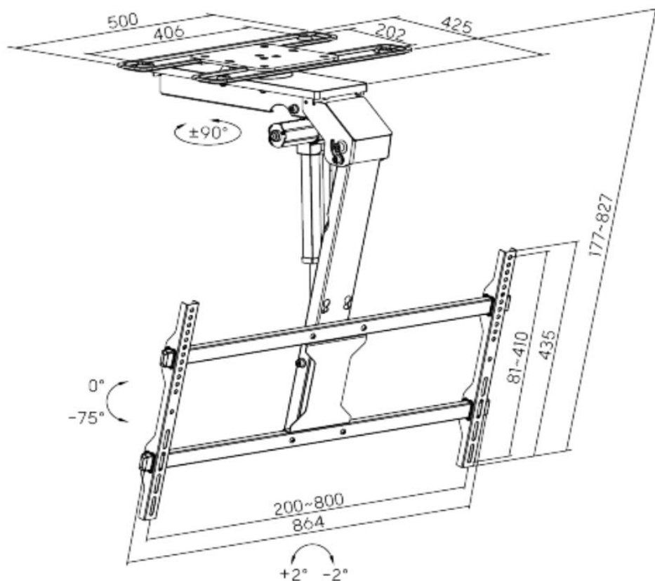
Dimensions (mm)
